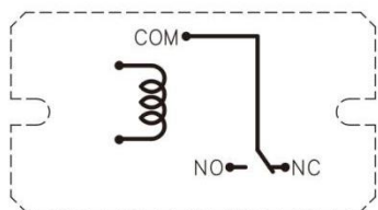
转换C型/Conversion C type
